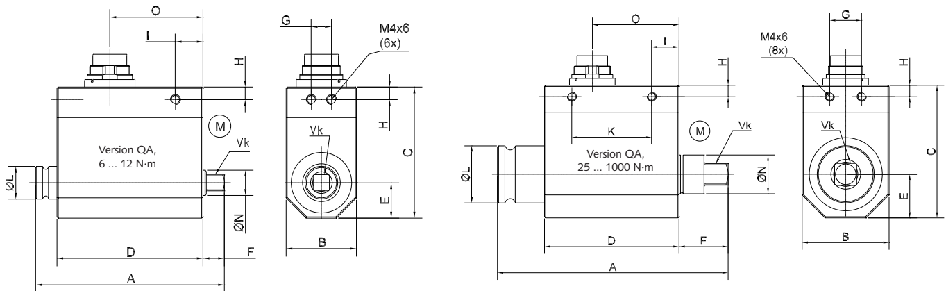
Dimensions Version QA (with rotational angle measurement)
